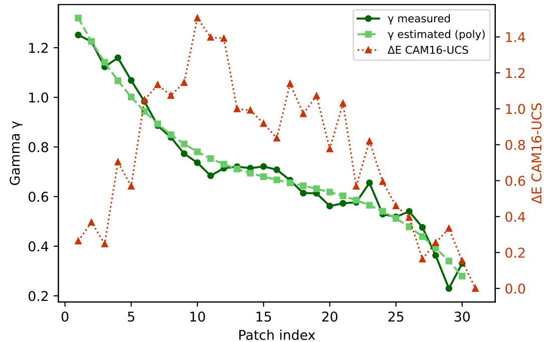
G — gamma (degree 3) mean \Delta E=0.753 std=0.404
